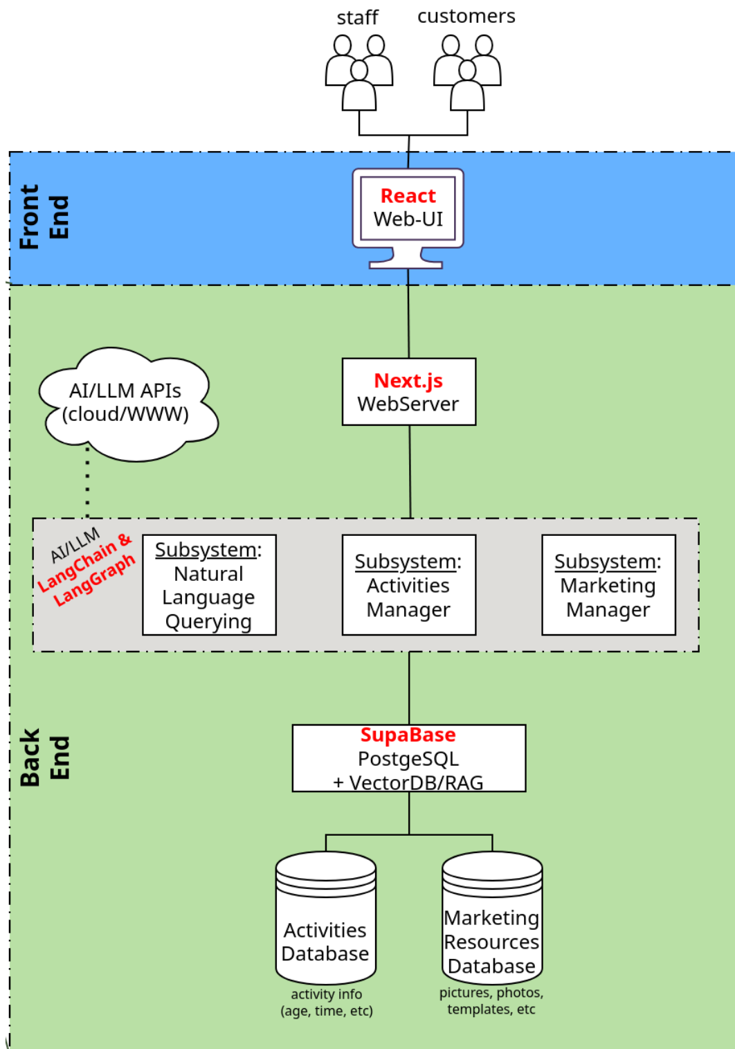
Tech Stack Overview
